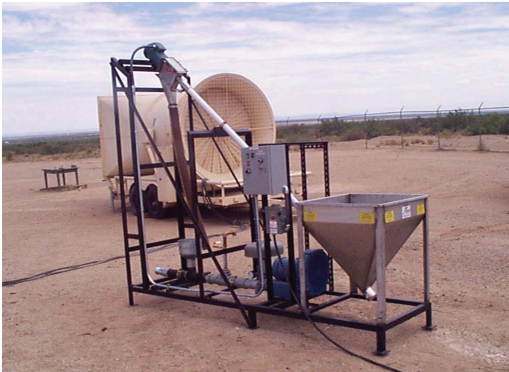
Figure 1. Typical Sand and Dust Injection System with 200 HP Wind Generator in Background
